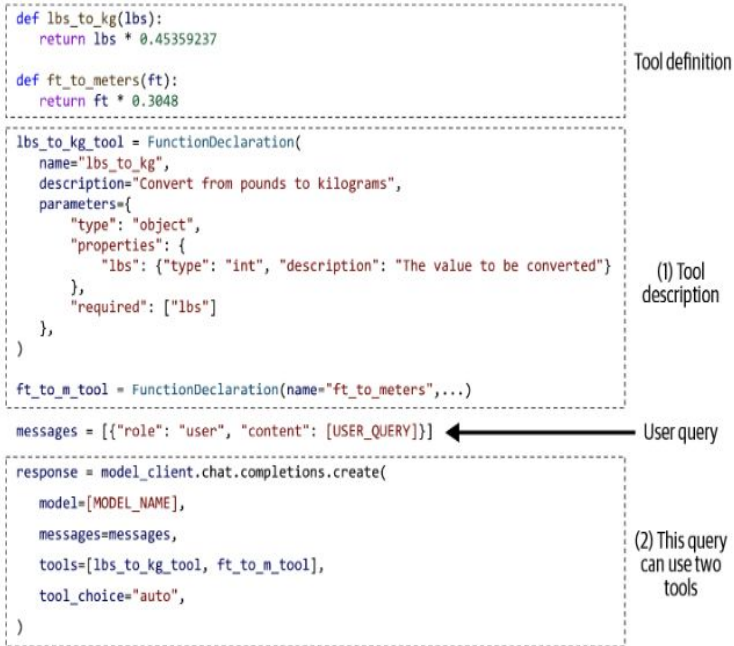
Figure 6-10. An example of a model using two simple tools.
