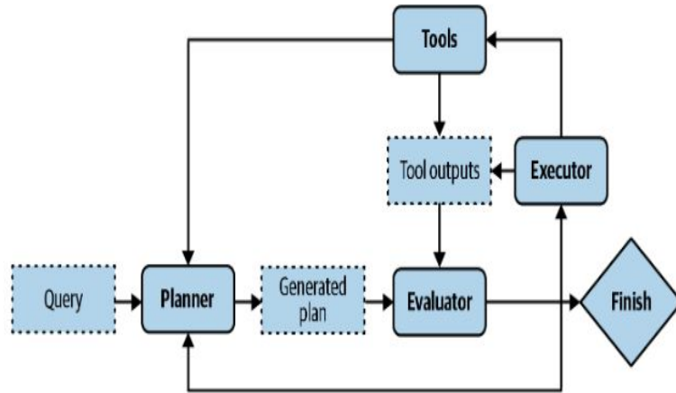
Figure 6-9. Decoupling planning and execution so that only validated plans are executed.
